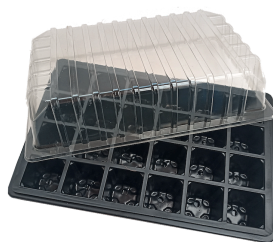
24-cell propagator
