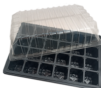
Propagator
